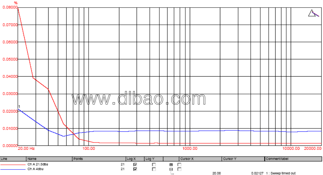
SY0907-2477A4 THD+N vs Frequency
